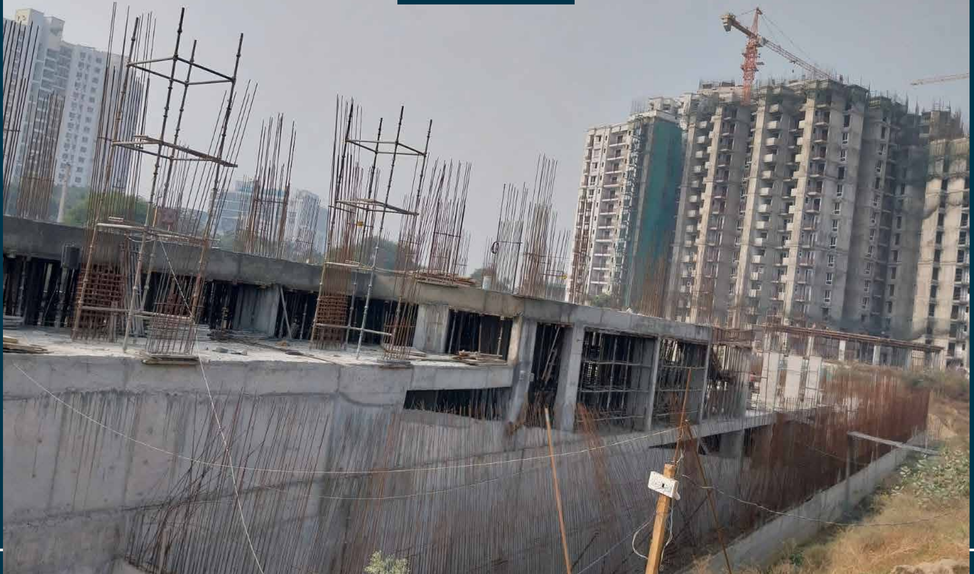
Underground floor slab casted
